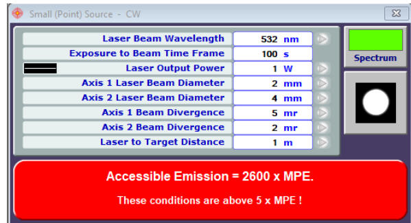
Figure 6: Defining Laser (adapted from LaserSafe PC)
