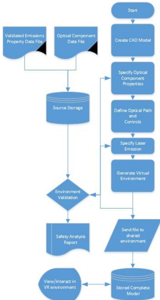
Figure 3: Data Flow in VERISA
