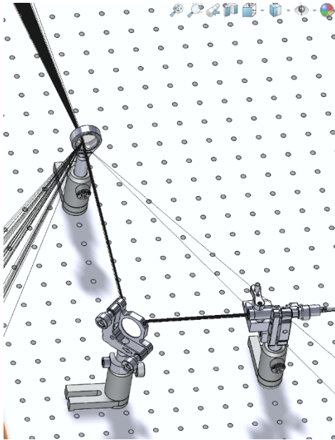
Figure 4: Misaligned Baseline Model
